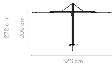
Sensu quattro diamond + grondverankering
