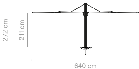
Sensu duo square + grondverankering
