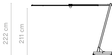
Kosmos shade round + concrete wheel base
